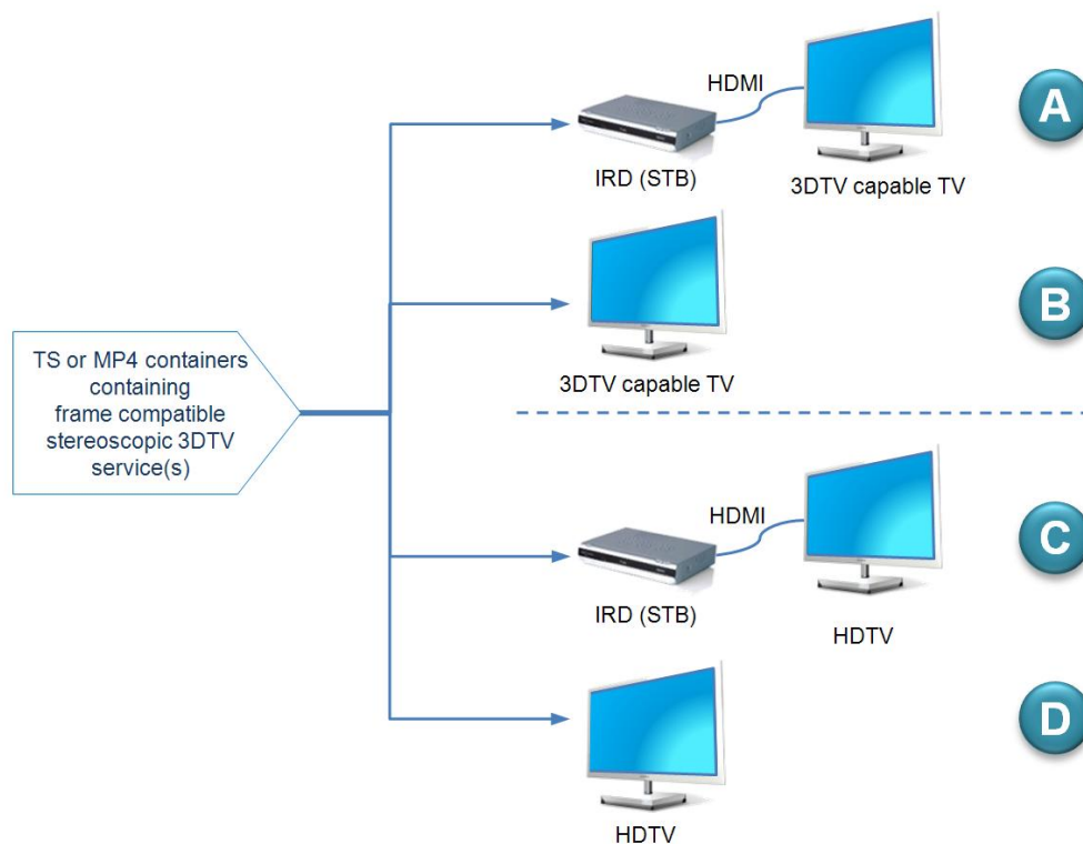
Figure 11: Frame compatible plano-stereoscopic 3DTV IRD use cases
